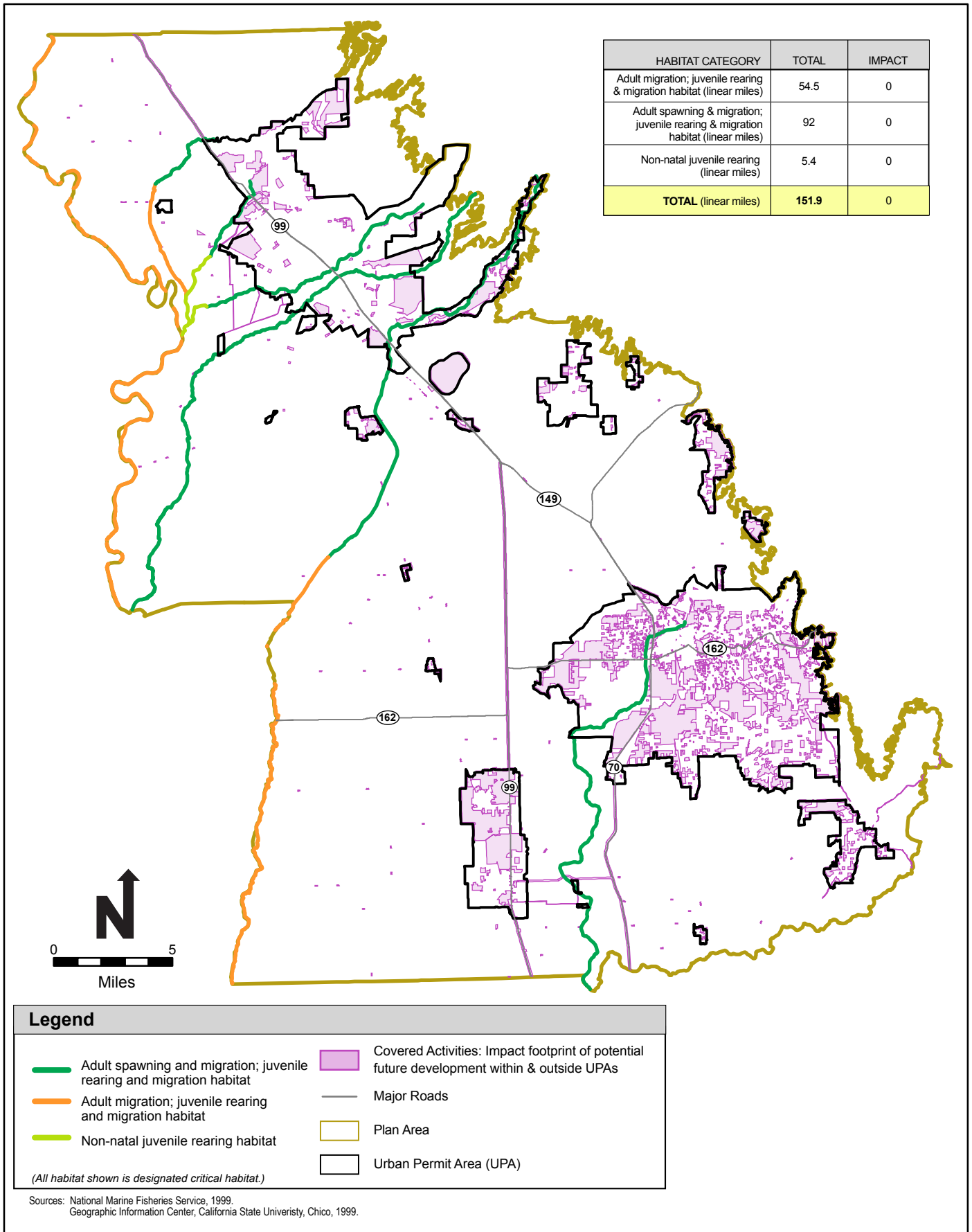
Figure 4-34. Central Valley Fall/Late-Fall Run Chinook Salmon: Direct Impacts of Covered Activities 6/7/11
