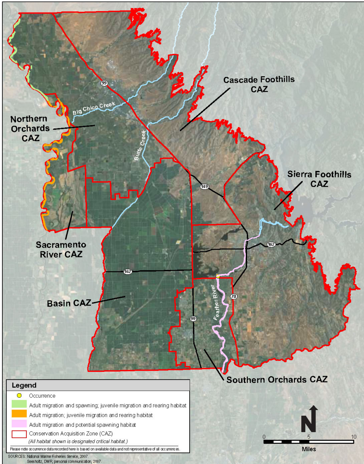
Figure A.20-1. Green Sturgeon Modeled Habitat and Recorded Occurrences
