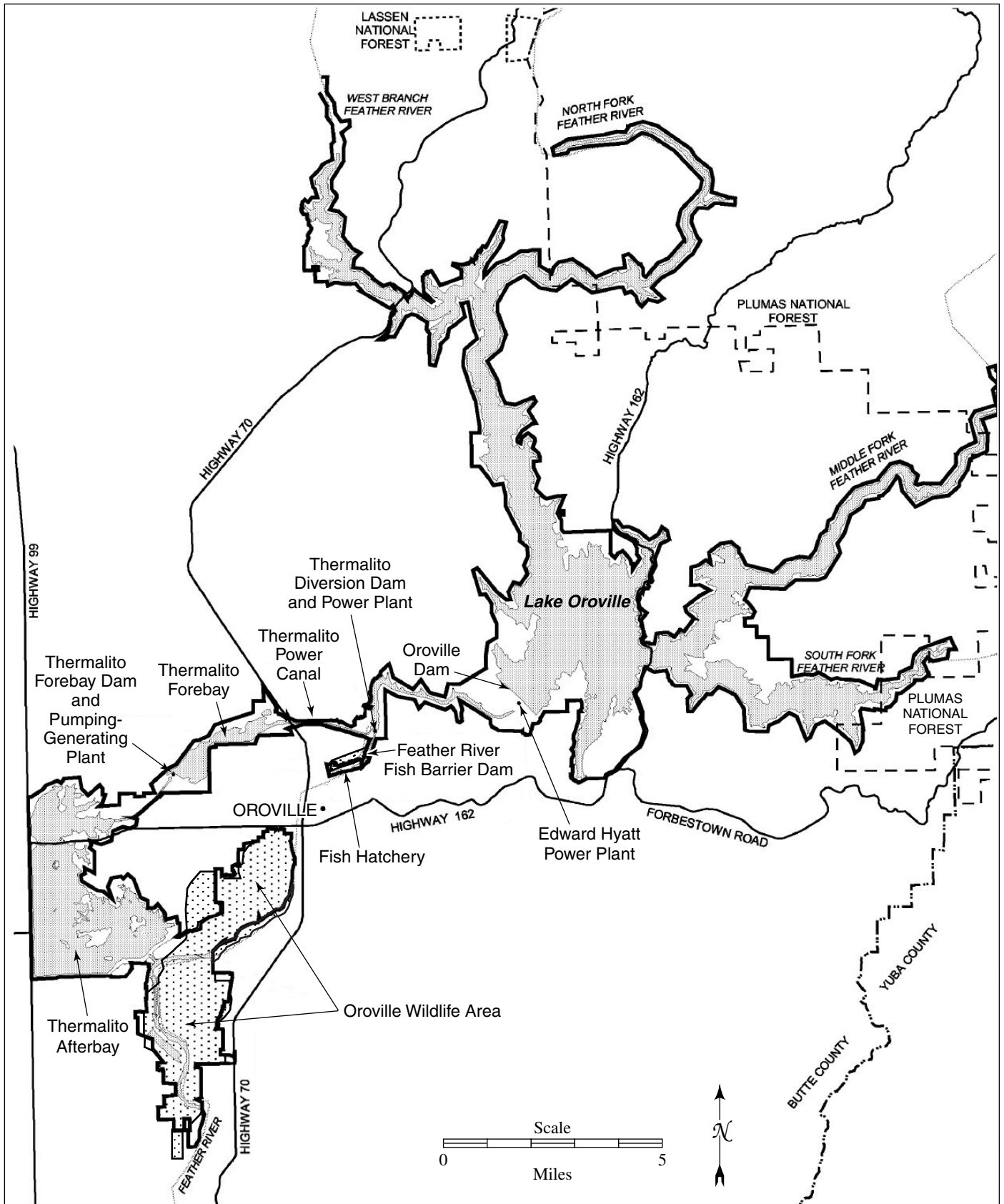
Figure 3-10. Lake Oroville Facilities: State Water Project
