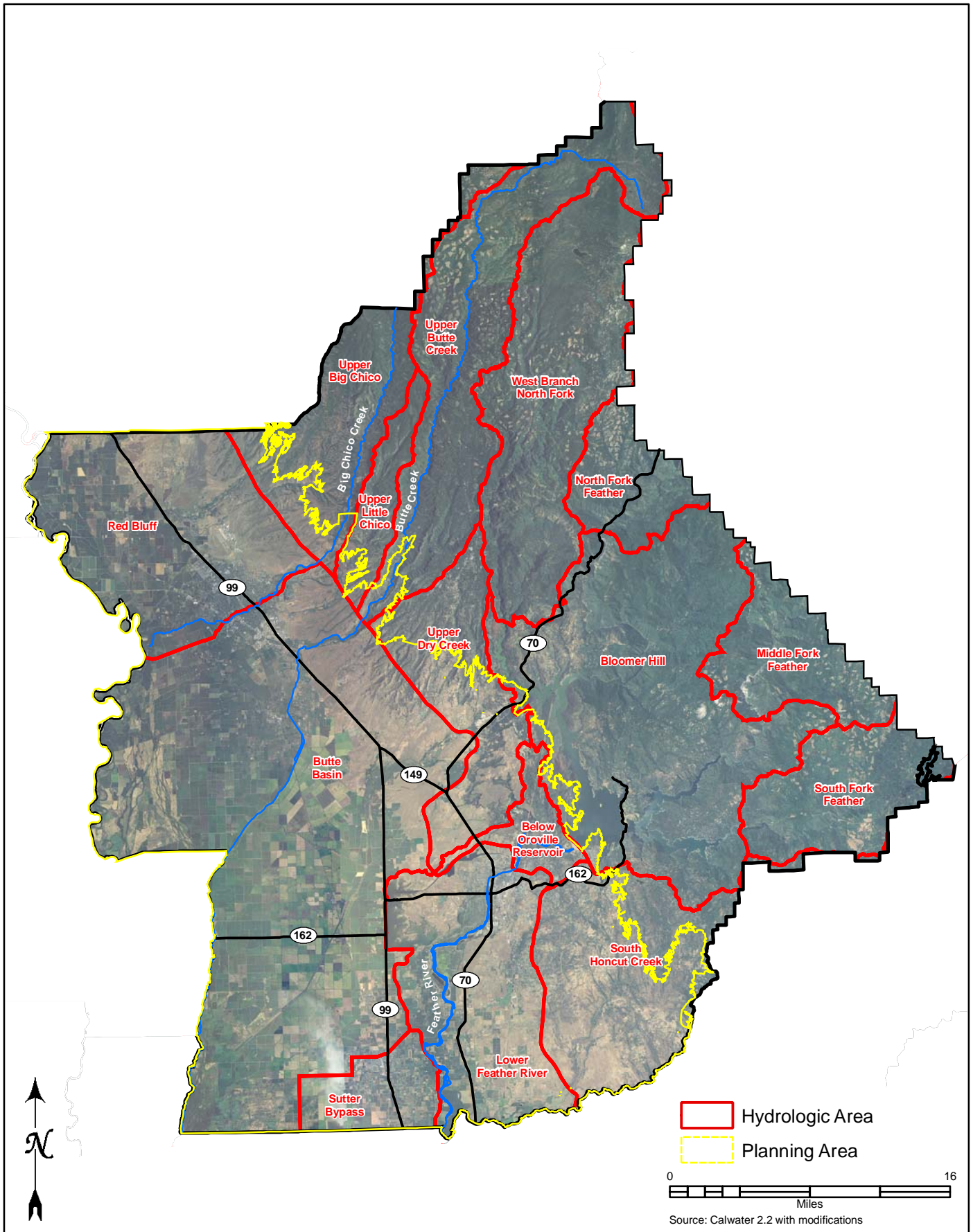
Figure 3-6. Hydrologic Areas within Butte County
